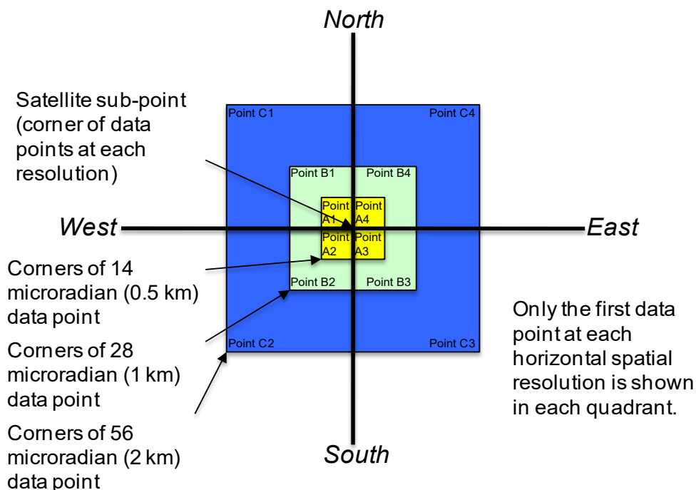
Figure 4.2.2-2 Fixed Grid Data Point Locations Relative to the Ideal Satellite Sub-Point (CCR-03893)
