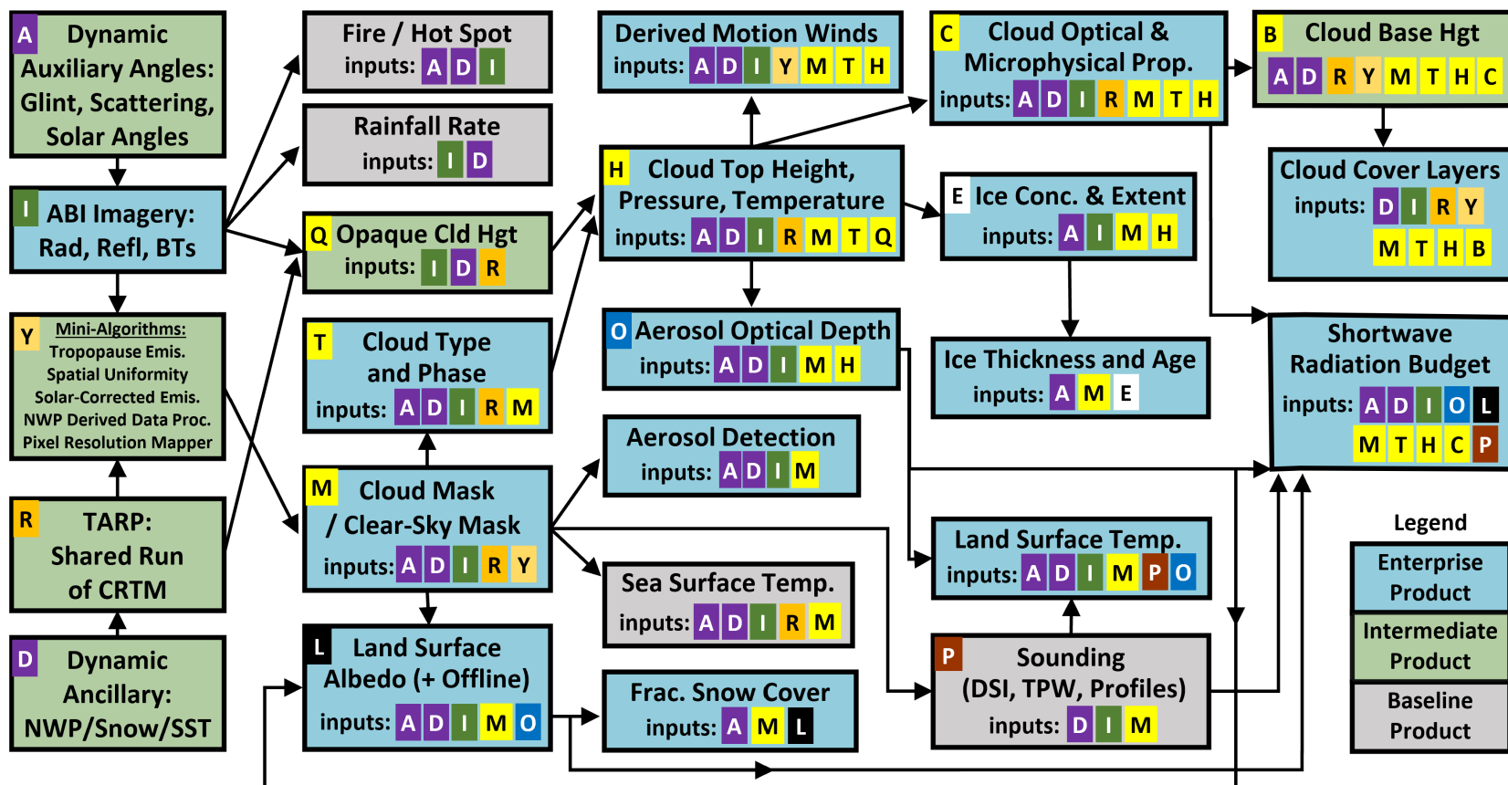
Figure 3.0 Level 2+ Algorithm Precedence Network
